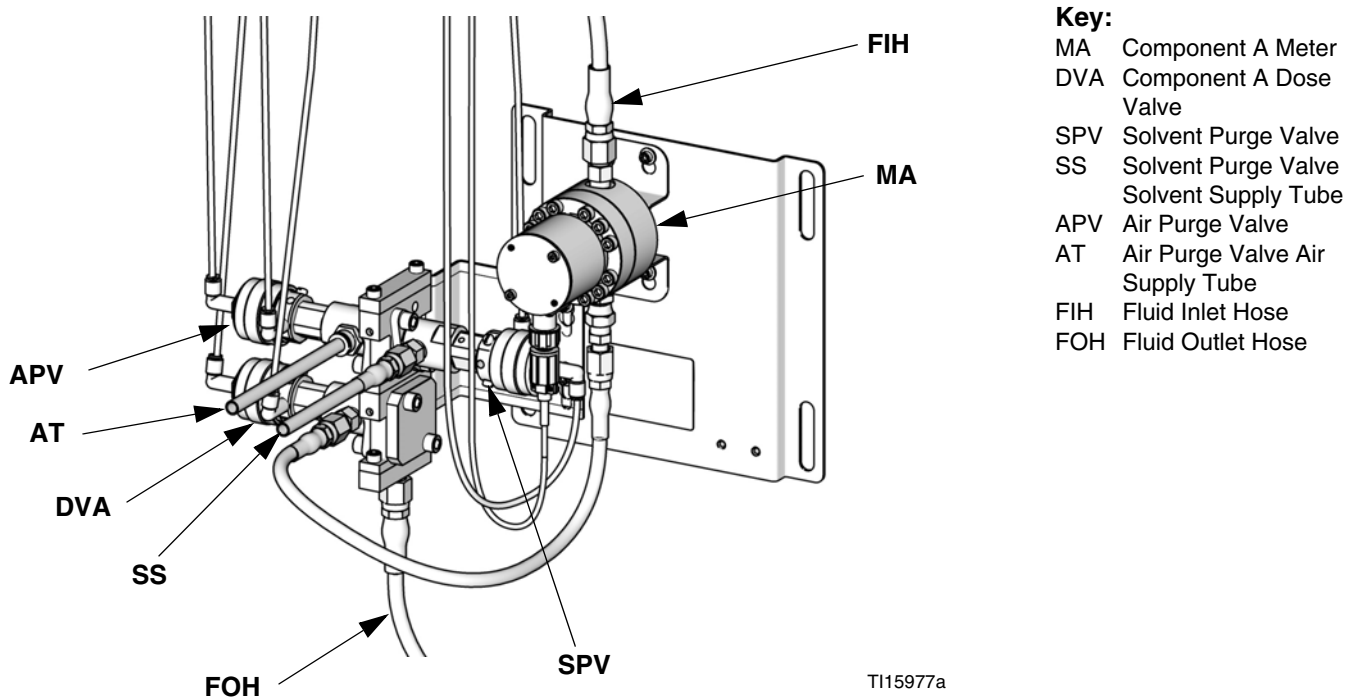
FIG. 108. Wall Mount Fluid Station
